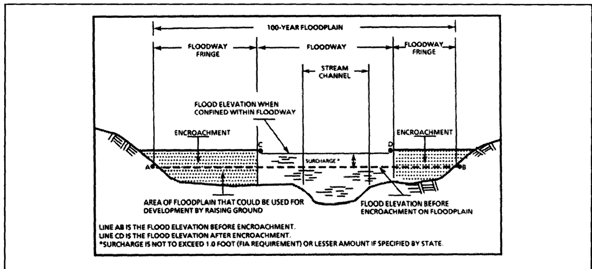
Figure 1. Floodway Schematic
